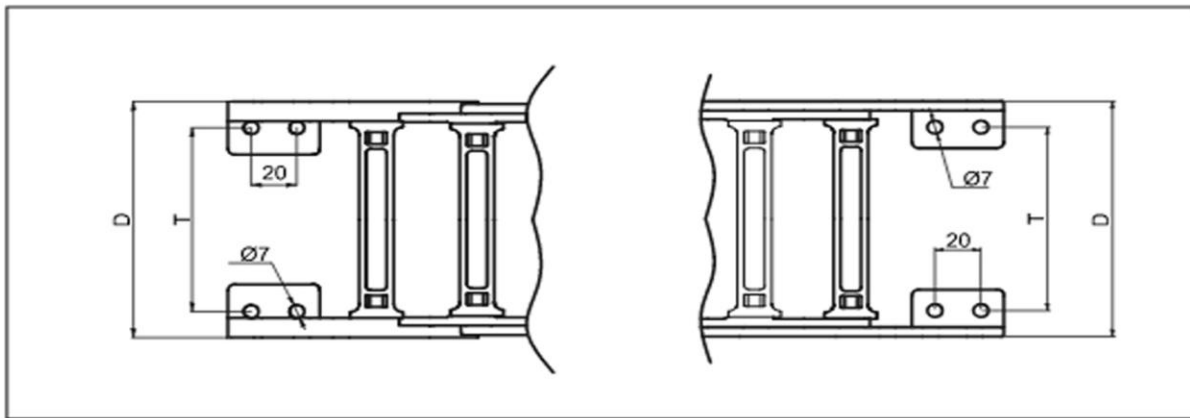
(Plastic End Brackets Connection)
